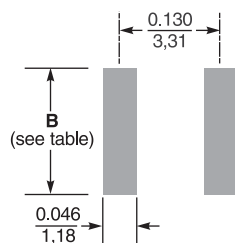
Suggested Land Pattern
